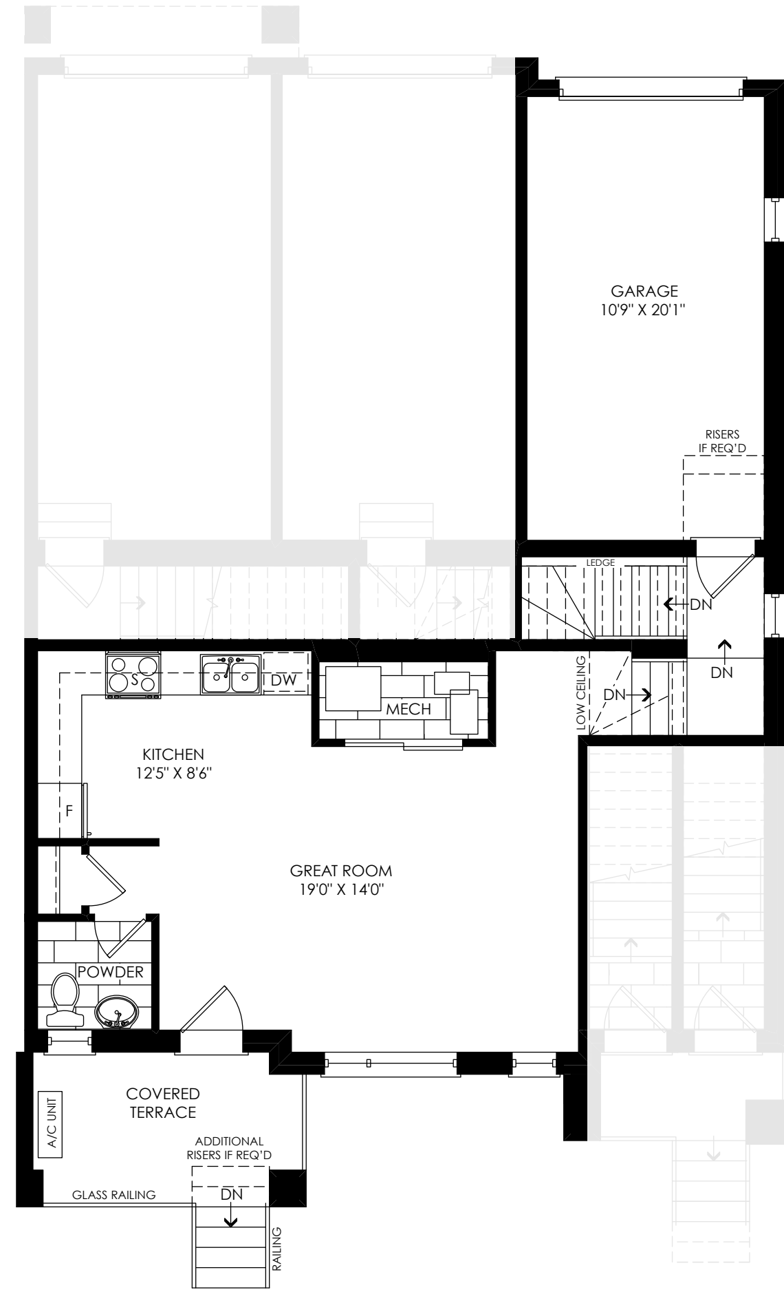
INTERIOR END UPGRADE MAIN FLOOR PLAN (FRONT)
