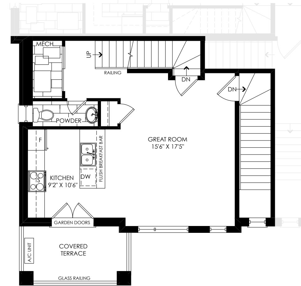
EXTERIOR UPGRADE SECOND FLOOR PLAN (FRONT)
