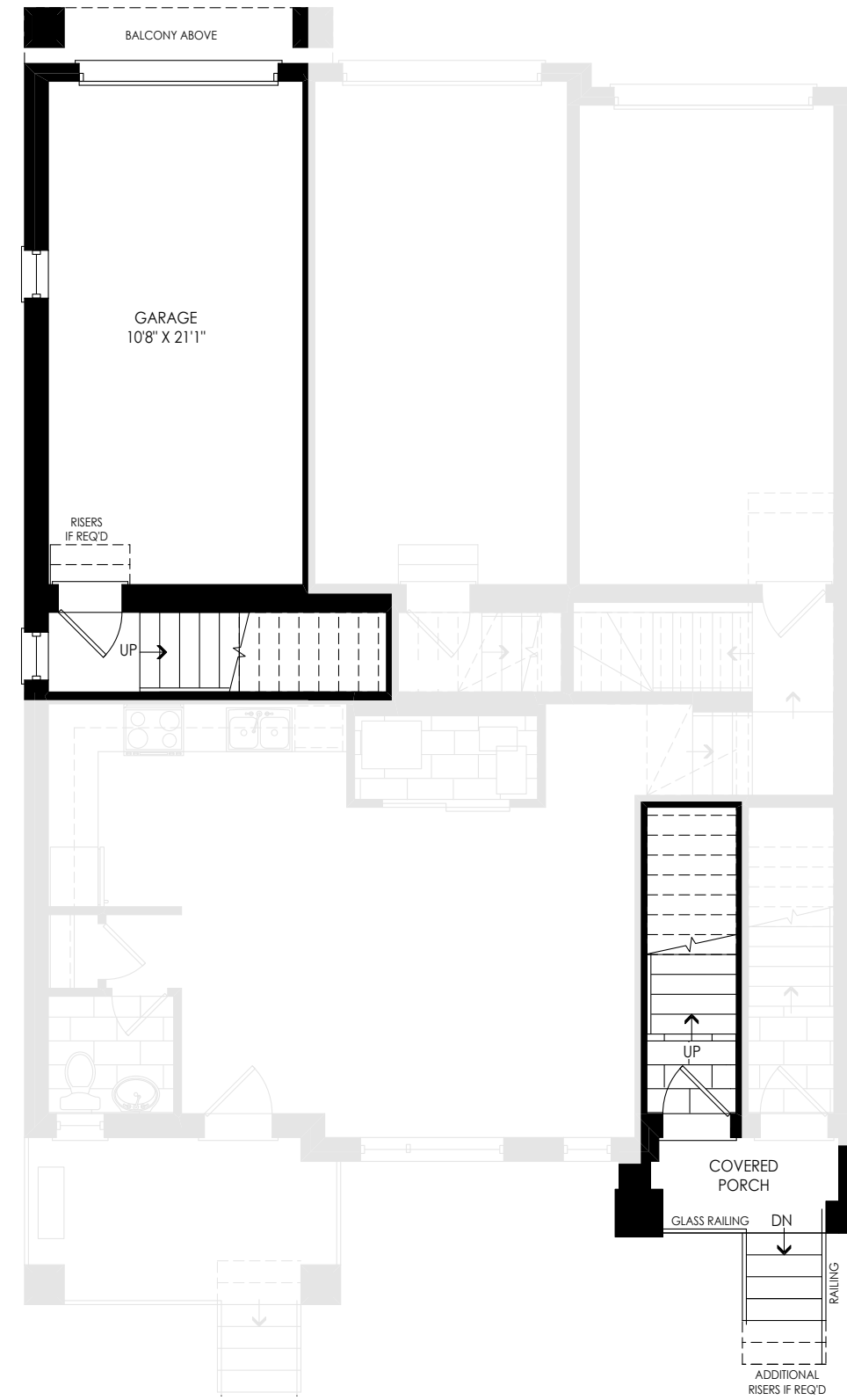
INTERIOR END MAIN FLOOR PLAN (FRONT)
