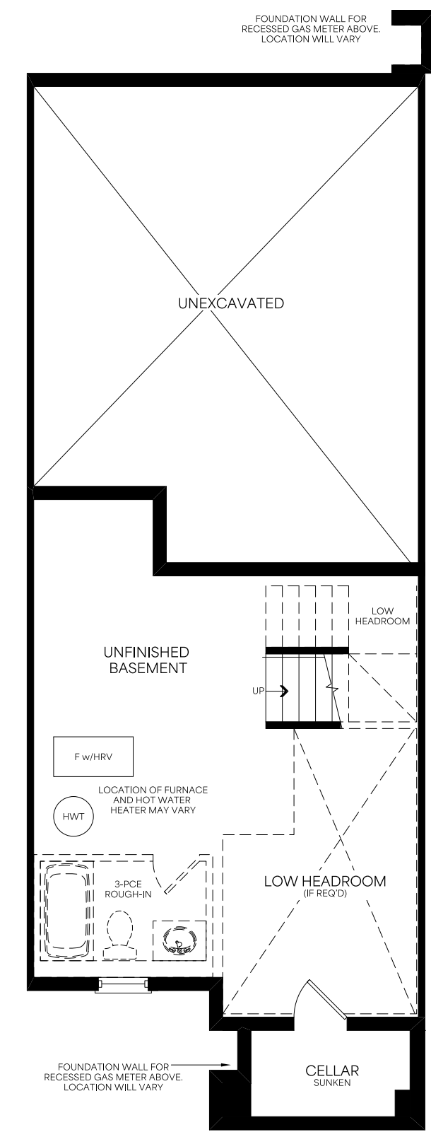
Basement Elevation C
