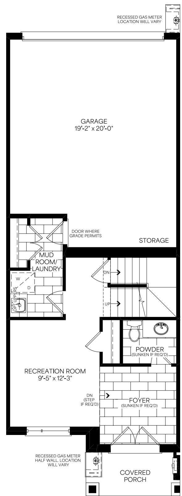
Ground Floor Elevation C
