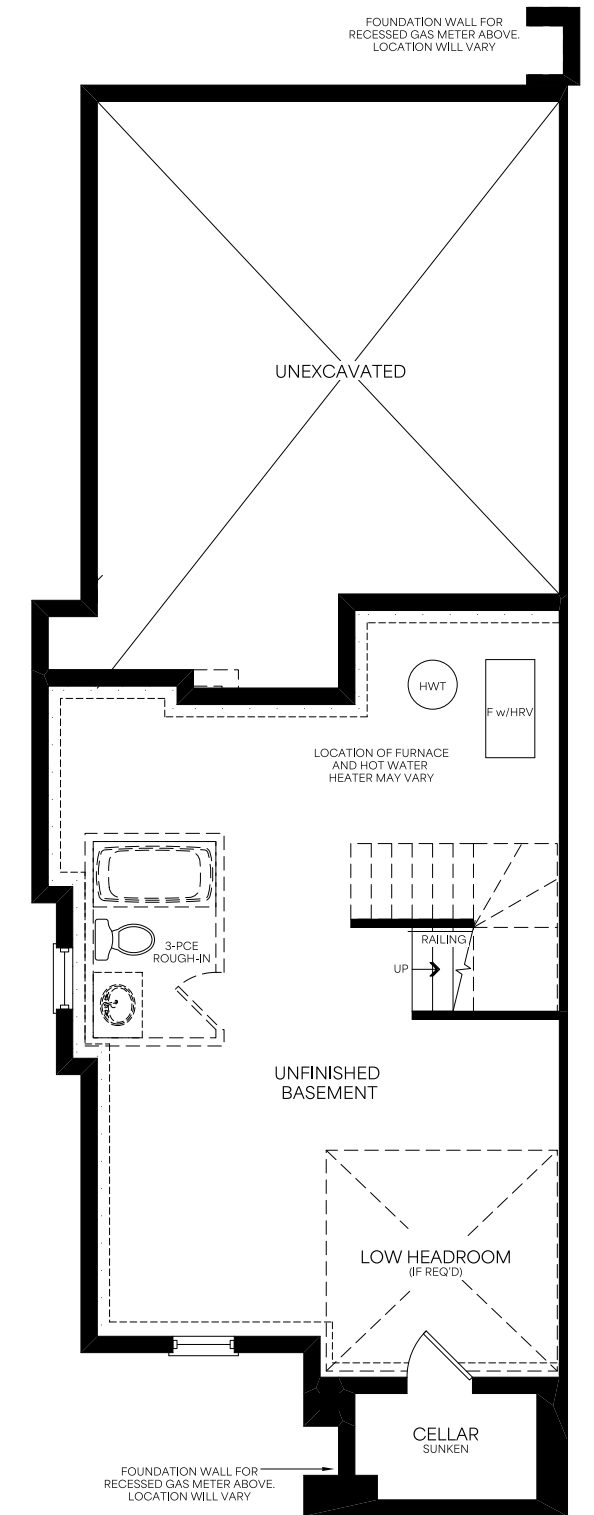
Basement Elevation C
