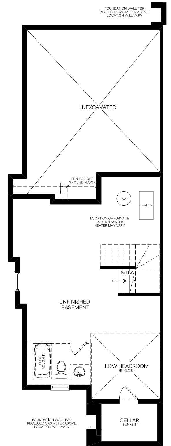
Basement Elevation B1
